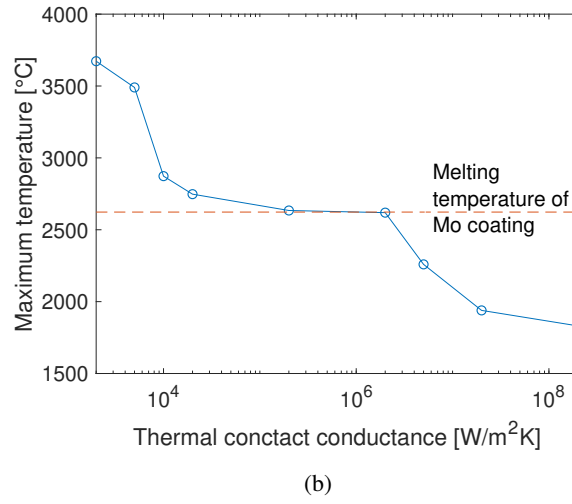
Figure 10. a) Temperature distribution in the molybdenum-coated graphite block after a grazing beam impact for a TCC_{Mo-Gr}^* = 2.00 \cdot 10^6 [W/m^2K] (half model considering YZ symmetry plane). b) Maximum temperature in the molybdenum coating under a grazing beam impact versus the thermal contact conductance between the coating and graphite substrate
