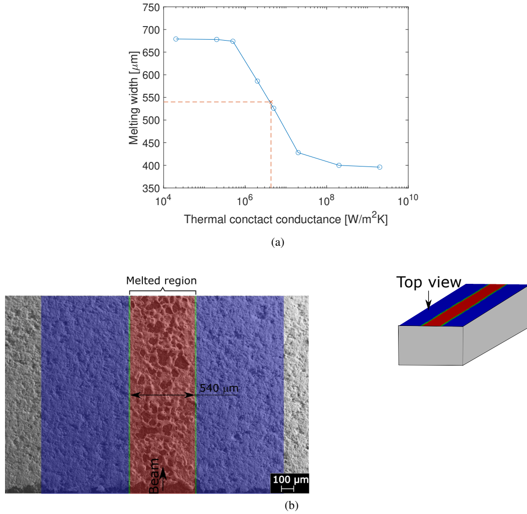
Figure 19. a) FEA findings for melted width of the copper coating at the beam entrance of the Cu-coated graphite block assuming a grazing impact as a function of the TCC (comparison of numerical and experimental findings at the orange marker). b) Superposition of the SEM image (black and white image) and numerical simulation (colour image, where melted region is in red and non-melted region is in blue) of the Cu coating (top view) for a TCC_{Cu-Gr}^* = 4.30 \cdot 10^6 [\text{W/m}^2\text{K}] (orange marker in previous graph a), showing the good agreement between simulations and experimental observations in terms of melted width.
